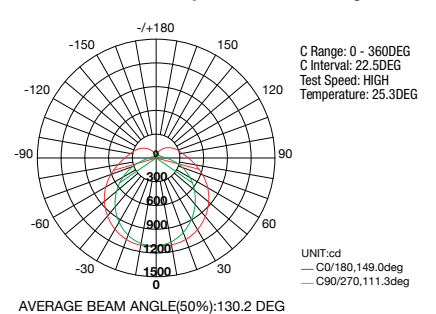
Luminous Intensity Distribution Diagram
