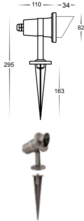
HV1431T Spike and surface mounted with hood
