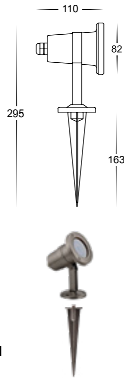
HV1432T Spike and surface mounted
