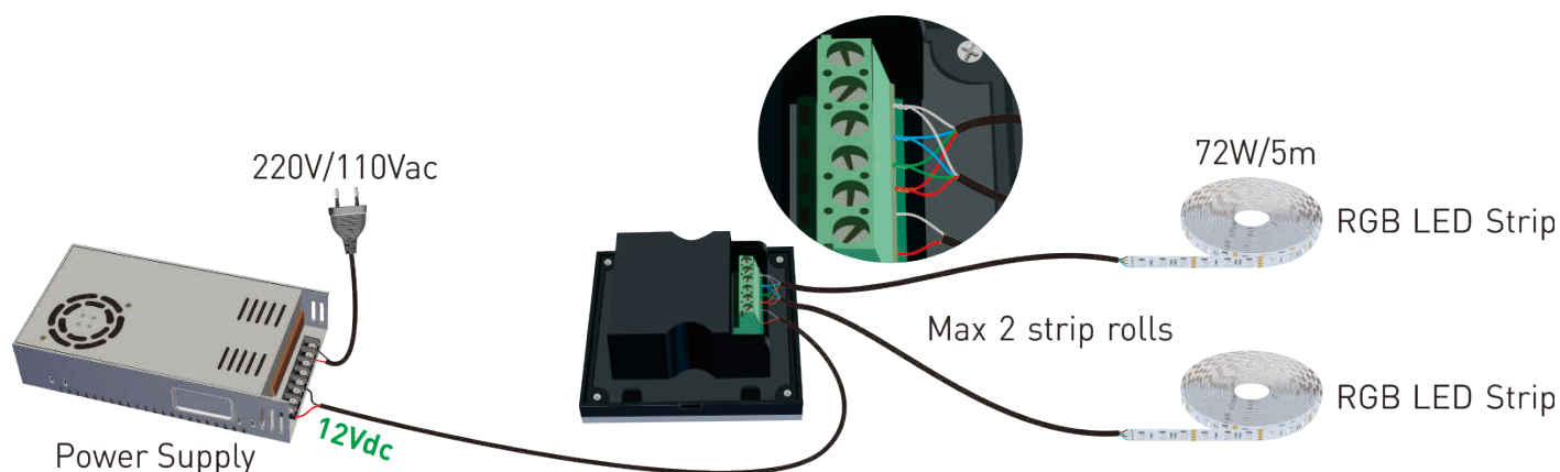
Sample wiring diagram
