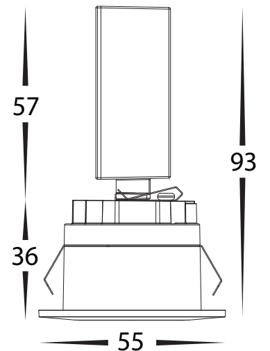
Cut Out: Ø45mm
