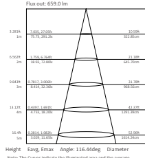
Beam diagram
