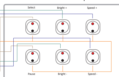
Reverse side of Switch plate
