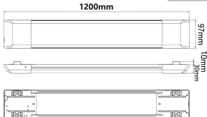
BATTENS001 - REAR
