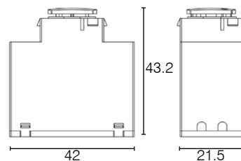
MASTER MECH
